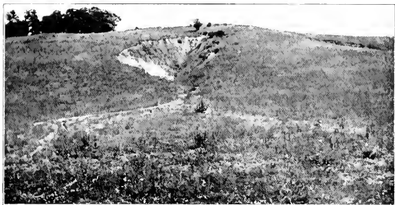
A. A young gully near Lacon. The material removed in the formation of the gully is spread upon the flat in the foreground, forming an alluvial fan.
